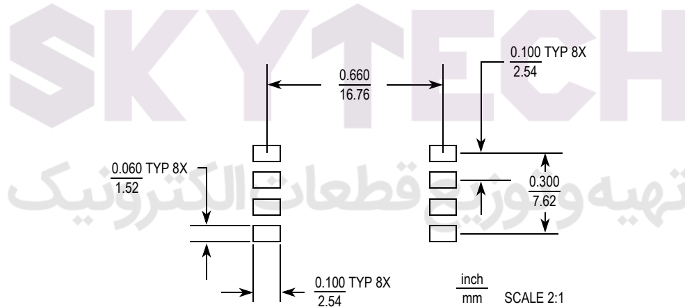
Figure 5. Small Outline Package Footprint
